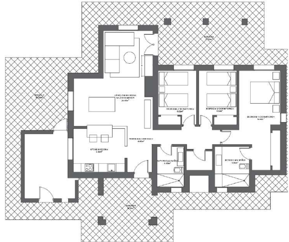
PLANTA BAJA GROUND LEVEL
