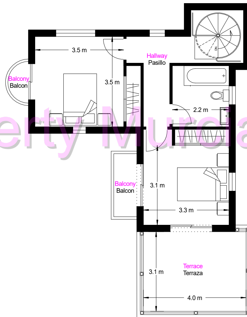
First floor/ Planta alta 50m2
